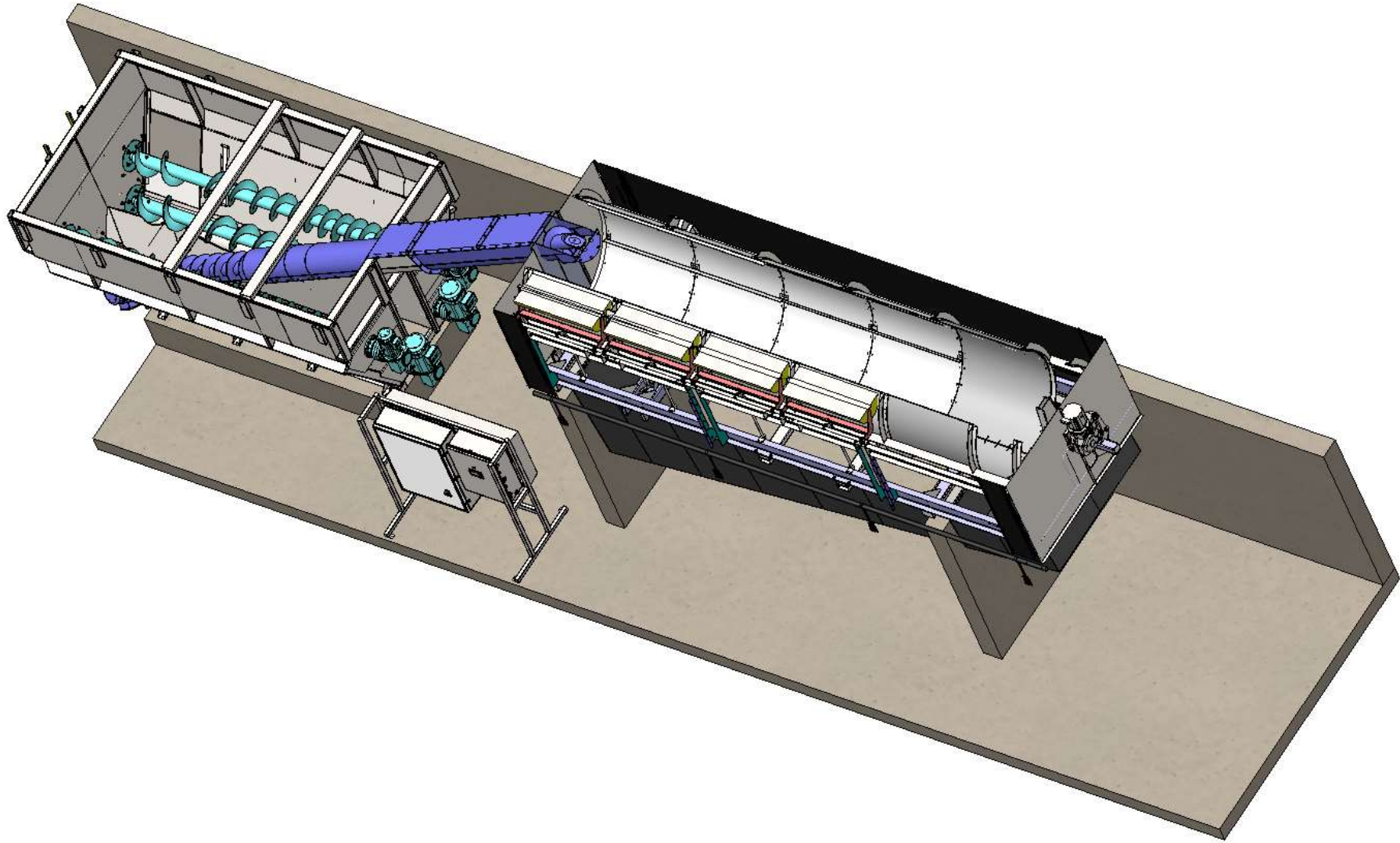
TROMMEL TOP SECTION VIEW *ROLL TARP OPEN – BOWS & TARP FRAME HIDDEN
